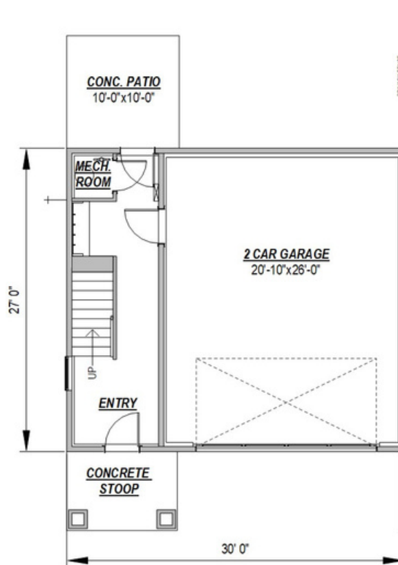
First Floor 233 SF
