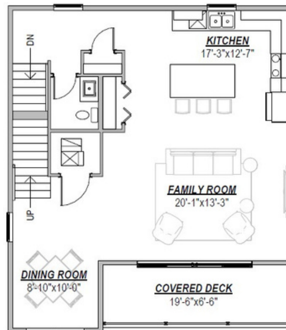
Second Floor 879 SF
